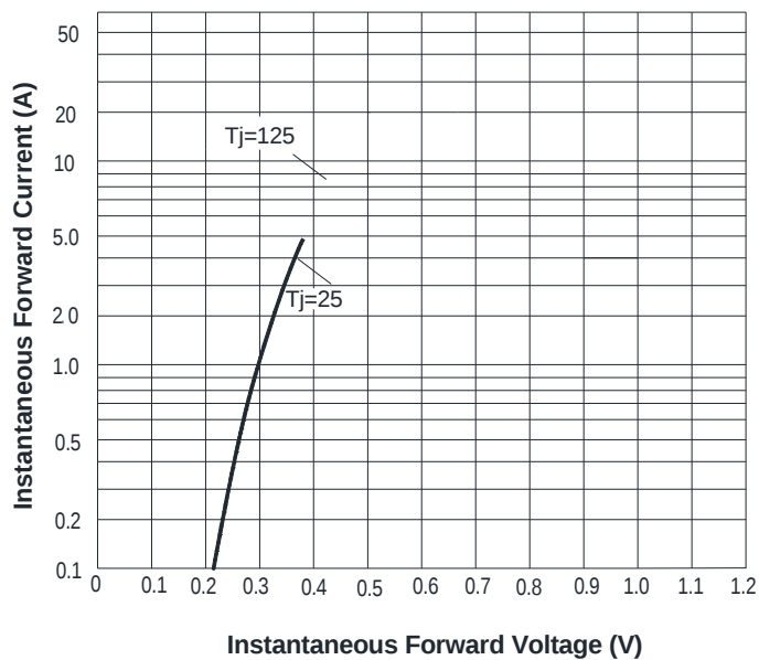
FIG3: Forward Voltage
