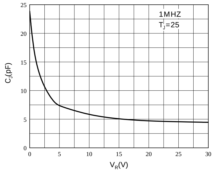
Fig.2: Capacitance Characteristics
