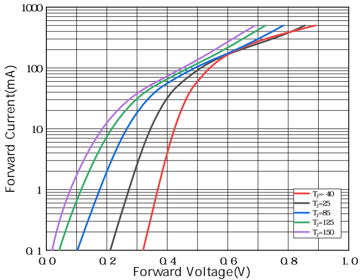
Fig.3: Forward Characteristics
