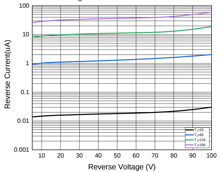
Fig.4: Reverse Characteristics
