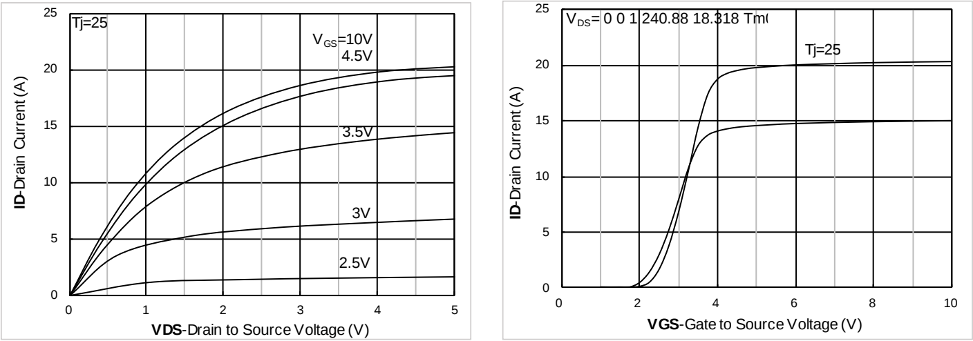
Figure 1. Output Characteristics;
