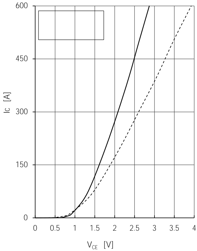
Fig1.IGBT Output Characteristics
