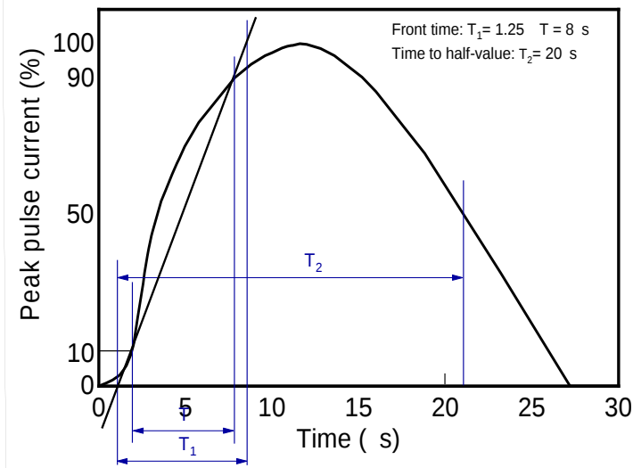
Fig.1 8/20 \mu s waveform per IEC61000-4-5
