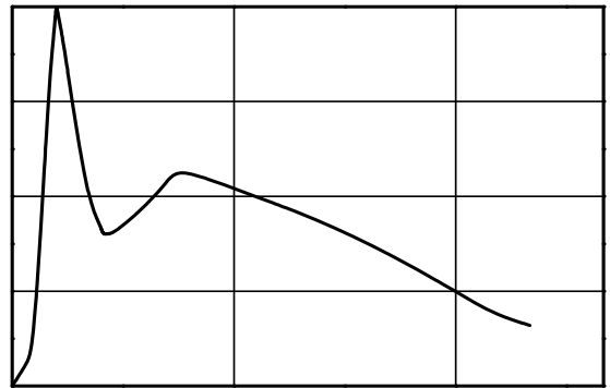
Contact discharge current waveform per IEC61000 # 2
